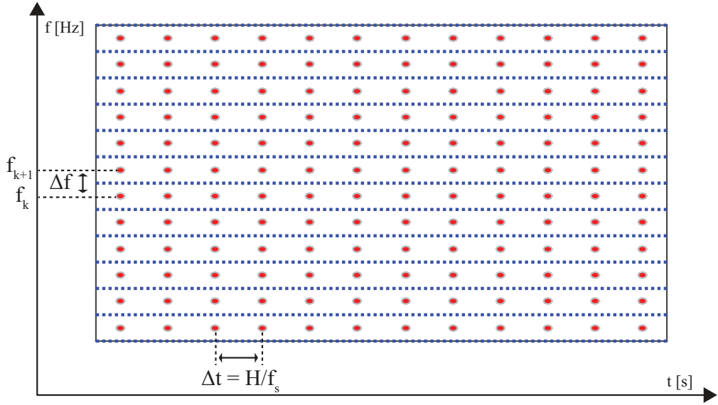
(a) FFT
